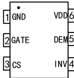
SOT23-6 Package
